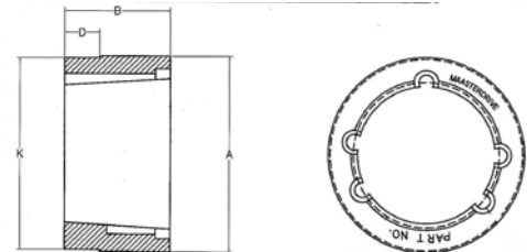
W Style TB Bushing Weld-On
